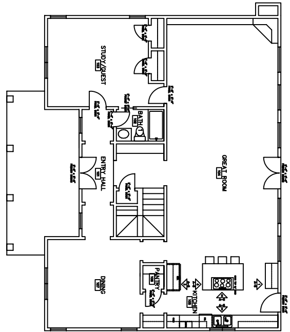
1 FIRST FLOOR SYMBOLS PLAN SCALE: 1/4" = 1'-0"
